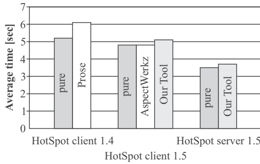
Figure 3: SPECjvm98 results.
